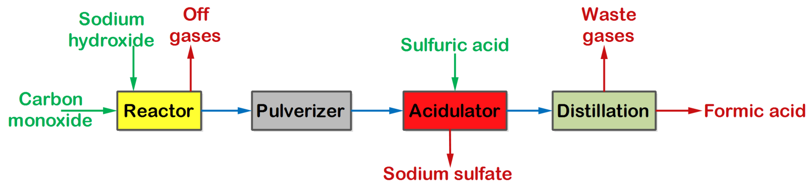
Figure: Manufacture of Formic acid from sodium formate
